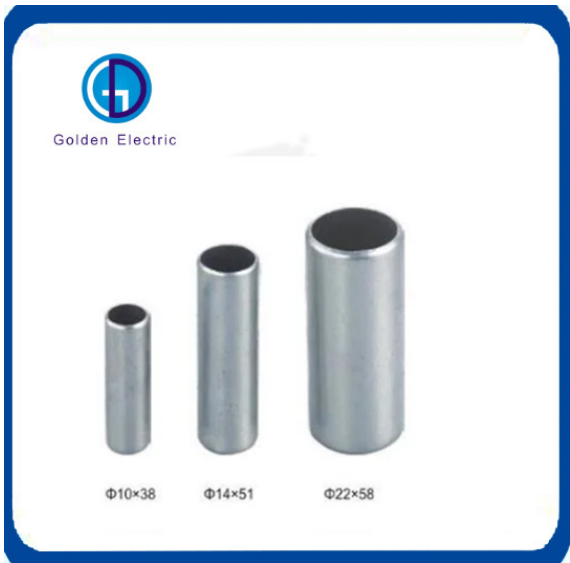
Copper Fuse Tube
