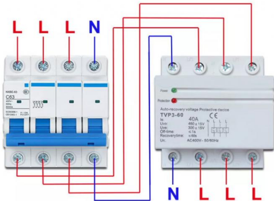
Circuit Breaker
