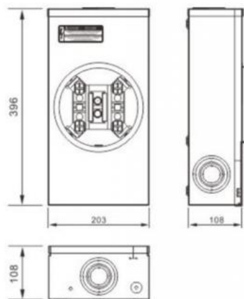
GD-200 Single phase type
