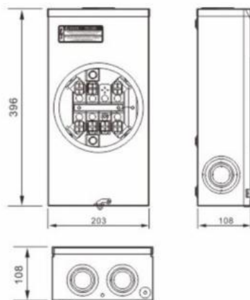
GD-200 Three phase type
