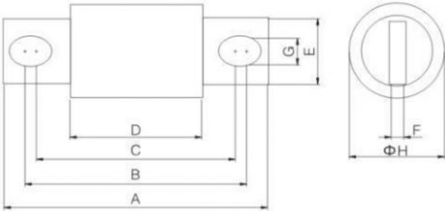
尺寸/Dimensions-mm
