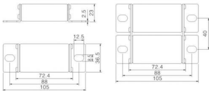
尺寸/Dimensions-mm
