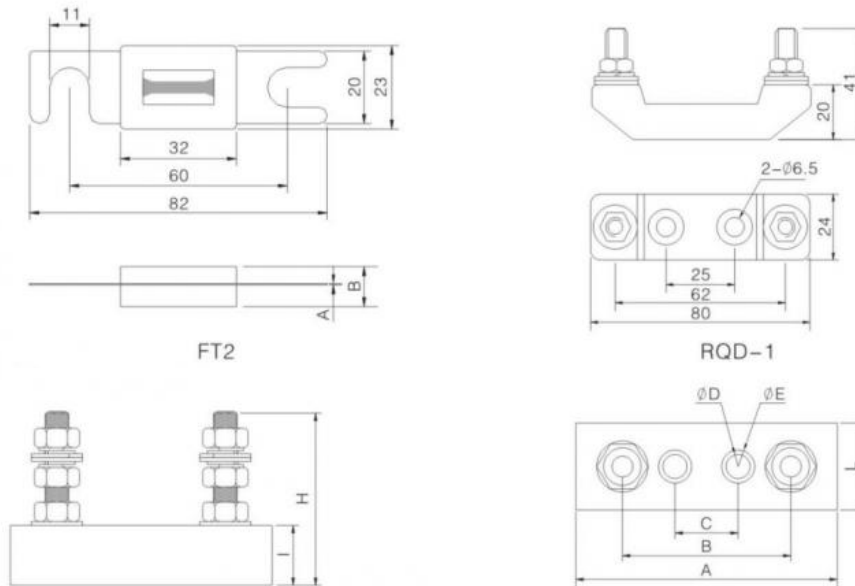
尺寸/Dimensions-mm
