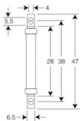
尺寸/Dimensions—mm
