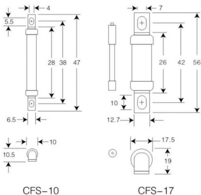
尺寸/Dimensions—mm
