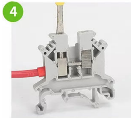
Rotate clockwise to clamp the wire Finally remove the screw driver
