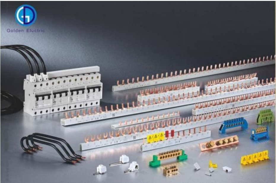
Fork Type 4-Phase busbar(M6)
