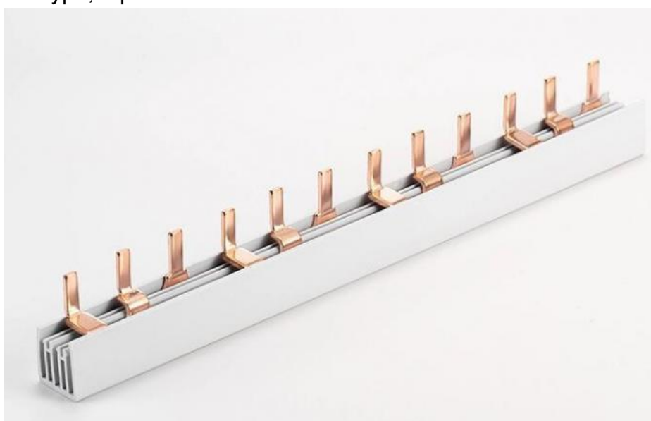
Pin type, 3 phase busbars
