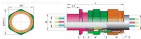
EX Standard Cable Gland JX6 Series - Metric, G Thread
