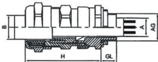
Ex Clamp Sealing Joint JX3- Metric, G Thread
