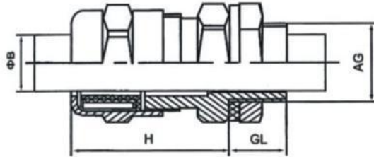
Double Sealed Explosion-proof Cable Gland JX2 - Metric Thread
