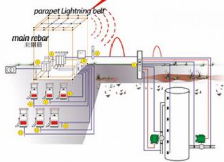
Building grounding system
