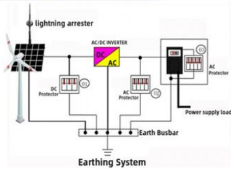
New energy power generation system
