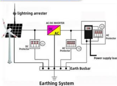
New energy power generation system
