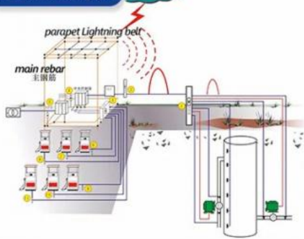
Petrochemical system
