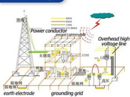
Mobile base station system
