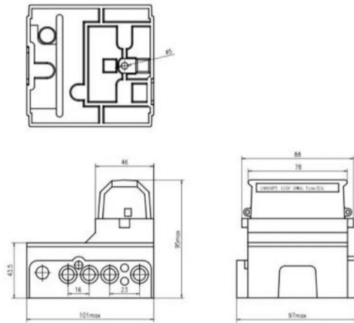
HRC100 II a/II b SPN (适配 II a、II b熔断体) (For II a、II b fuselink)
